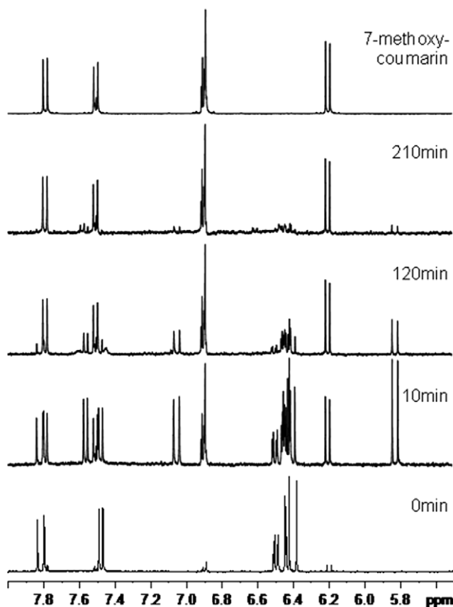
Figure 1. ^1\text{H} NMR spectra showing the transformation of MCIN into MCOUM (duration of photoirradiation in minutes: 0, 10, 120, and 210). A spectrum of an authentic MCOUM is presented at the top for reference.
