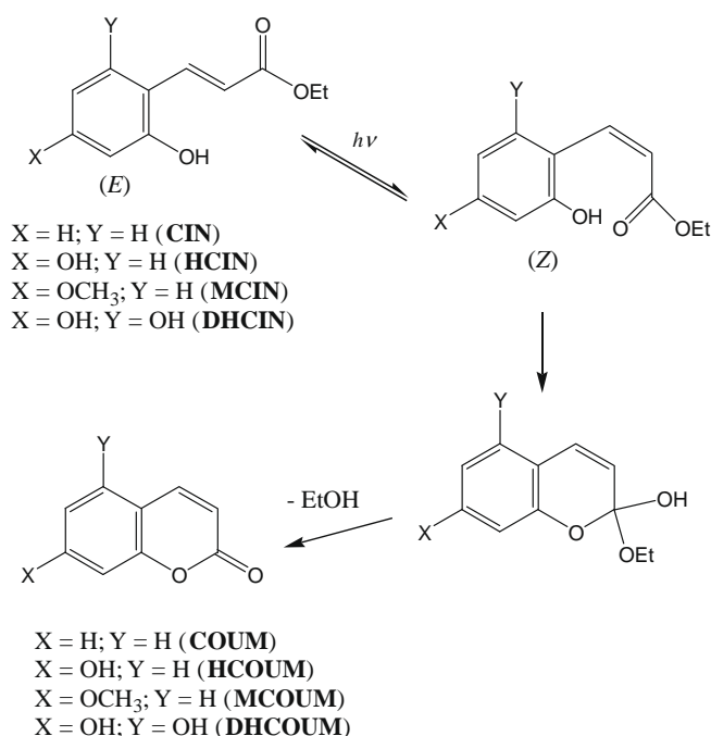
Scheme 1. Photoconversion of ( E )- o -hydroxycinnamates to coumarins.
