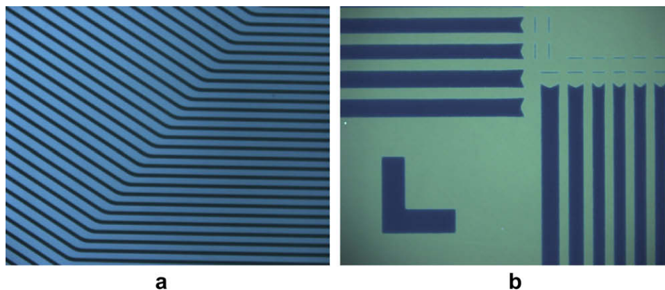
Figure 5. Fluorescent images obtained with 0.50- \mu\text{m} thick PMMA films containing (a) CIN and (b) MCIN (mass ratio of cinnamate:PMMA = 1:2.33 and mole ratio of cinnamate:TSA = 1.0.2). The actual colors may slightly differ because of computer image processing. Width of the long, dark lines in the images is 30 \mu\text{m} .
