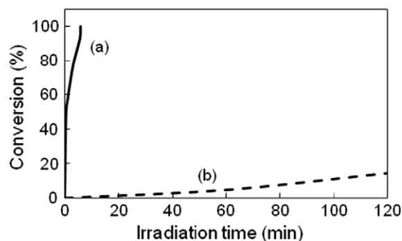
Figure 2. A plot of conversions of MCIN in PMMA films versus irradiation time: (a) in the presence of TSA (mole ratio of MCIN:TSA = 1:0.2), and (b) without TSA. The mass ratio of MCIN:PMMA was 1:2.33 and the films were prepared by casting.
