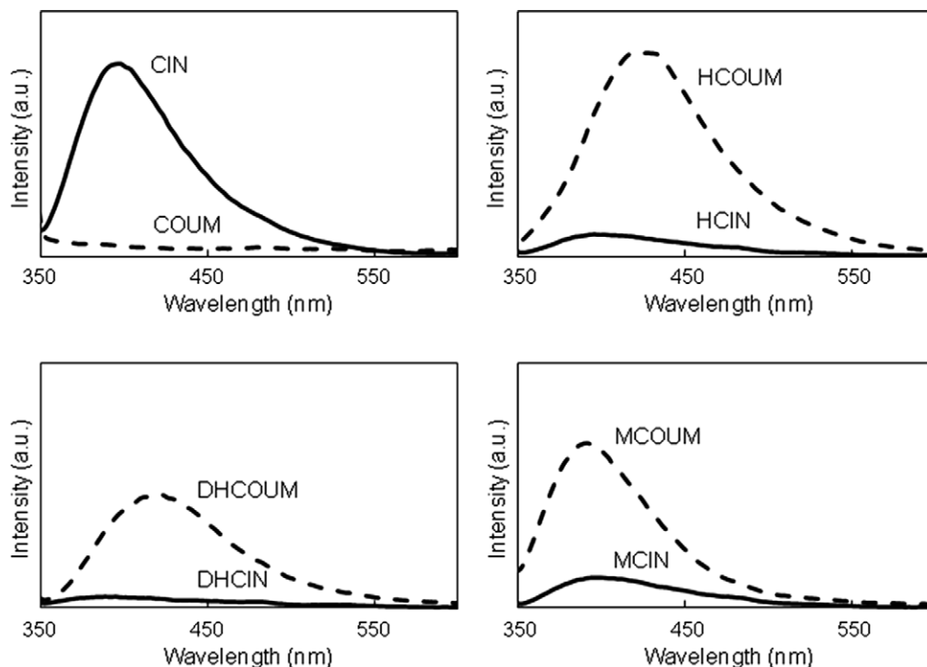
Figure 4. Emission spectra of cinnamates and coumarins. The films were prepared at a concentration of 9.10 \times 10^{-5} mol of cinnamate (or coumarin) in 0.070 g of PMMA by spin coating (film thickness: 0.43–0.51 \mu\text{m} , excitation wavelength: 330 nm).
