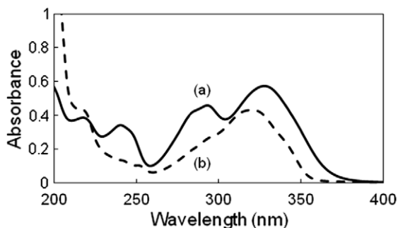
Figure 3. Optical absorption spectra of PMMA films containing (a) MCIN and (b) MCOUM. The films were prepared at a concentration of 9.10 \times 10^{-5} mol of MCIN or MCOUM in 0.070 g of PMMA by spin coating (film thickness: (a) 0.51 \mu\text{m} ; (b) 0.45 \mu\text{m} ).
